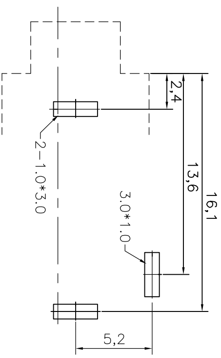
P.C.B. HOLE LAYOUT (BOTTOM VIEW)
